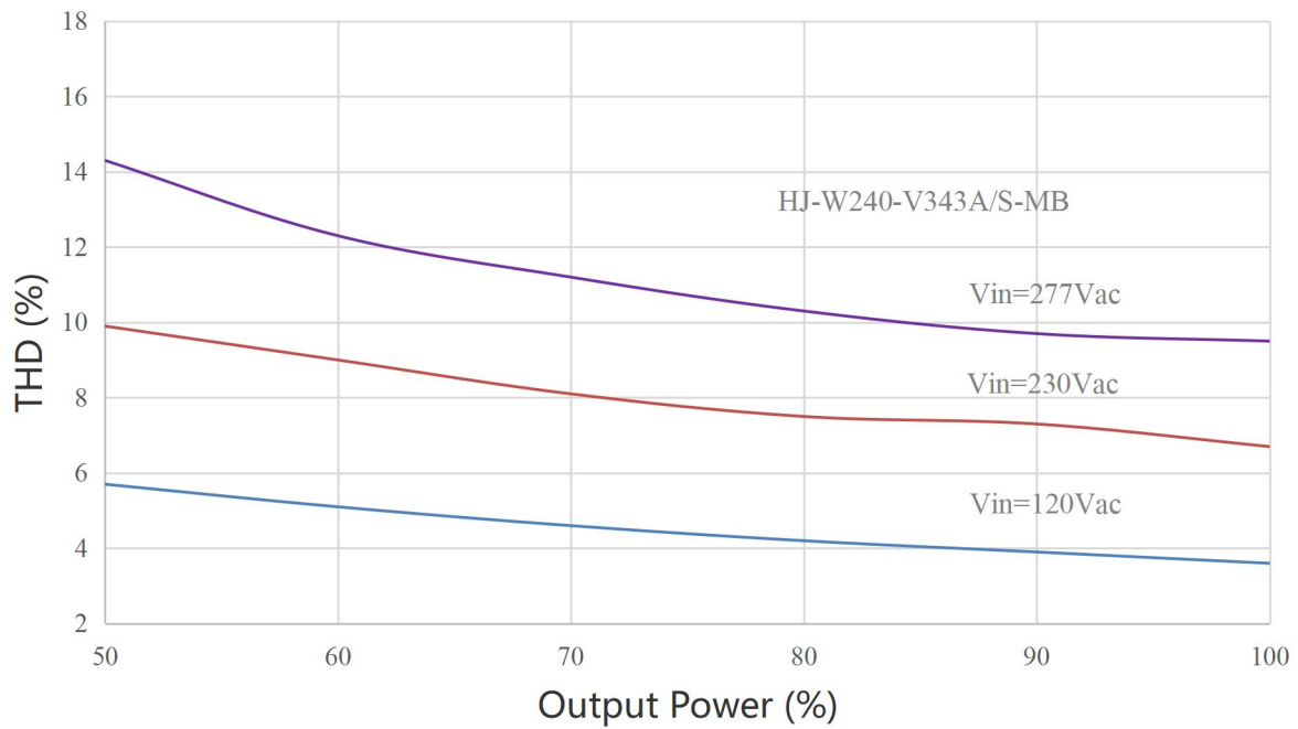
Fig 7. THD VS Output Power
