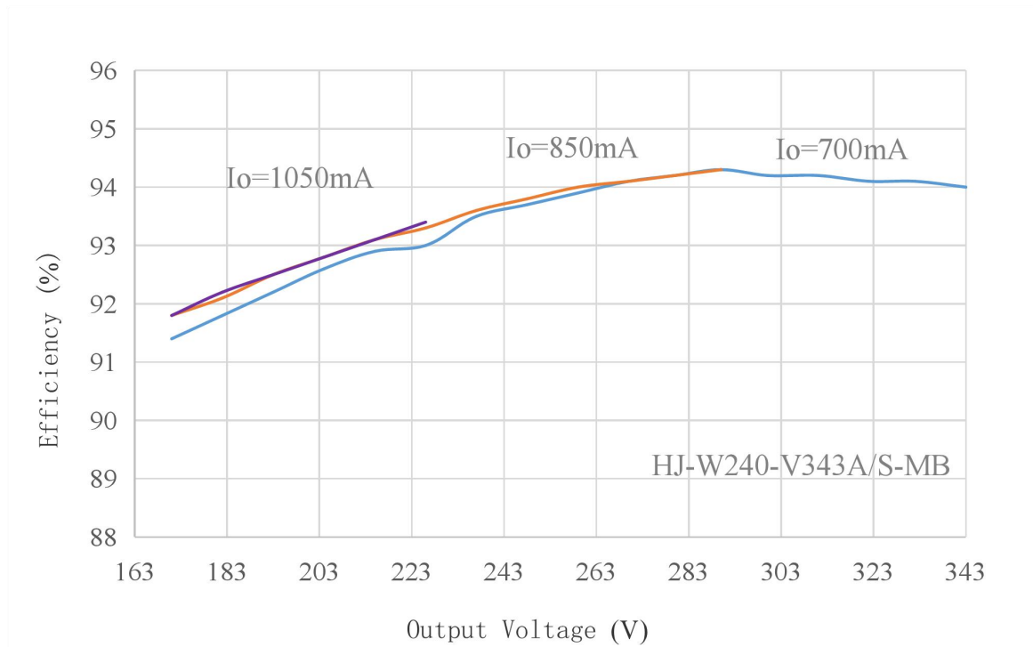
Fig. 3. Efficiency VS Output Voltage
