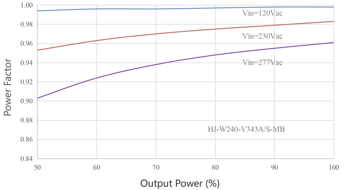
Fig 5. Power Factor VS Out Power
