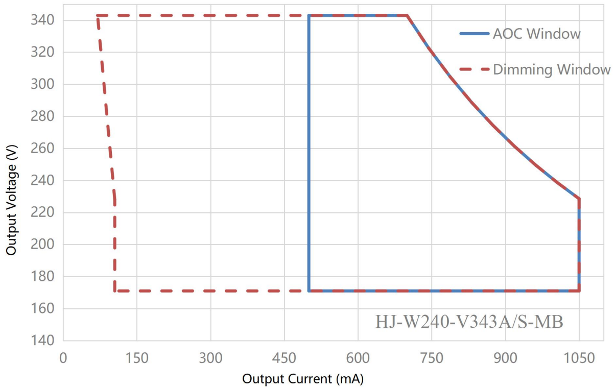
Fig 9. Output Voltage VS Output Current (Dimming/AOC Window)
