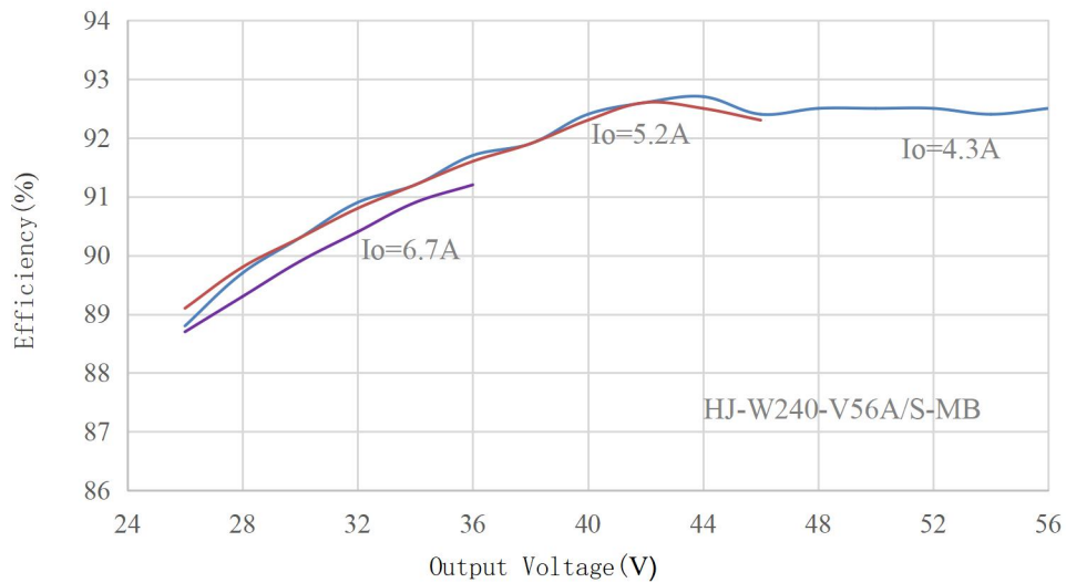
Fig.2. Efficiency VS Output Voltage
