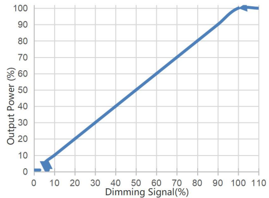
Fig 11. Output Power VS Dimming Signal
