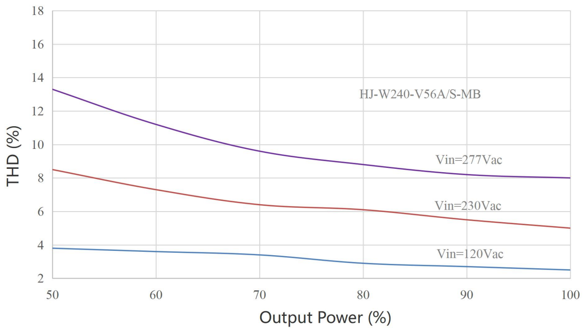
Fig.6 THD VS Output Power
